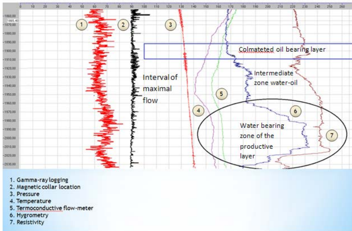
Fig. 8 Results of geophysical studies of the well
