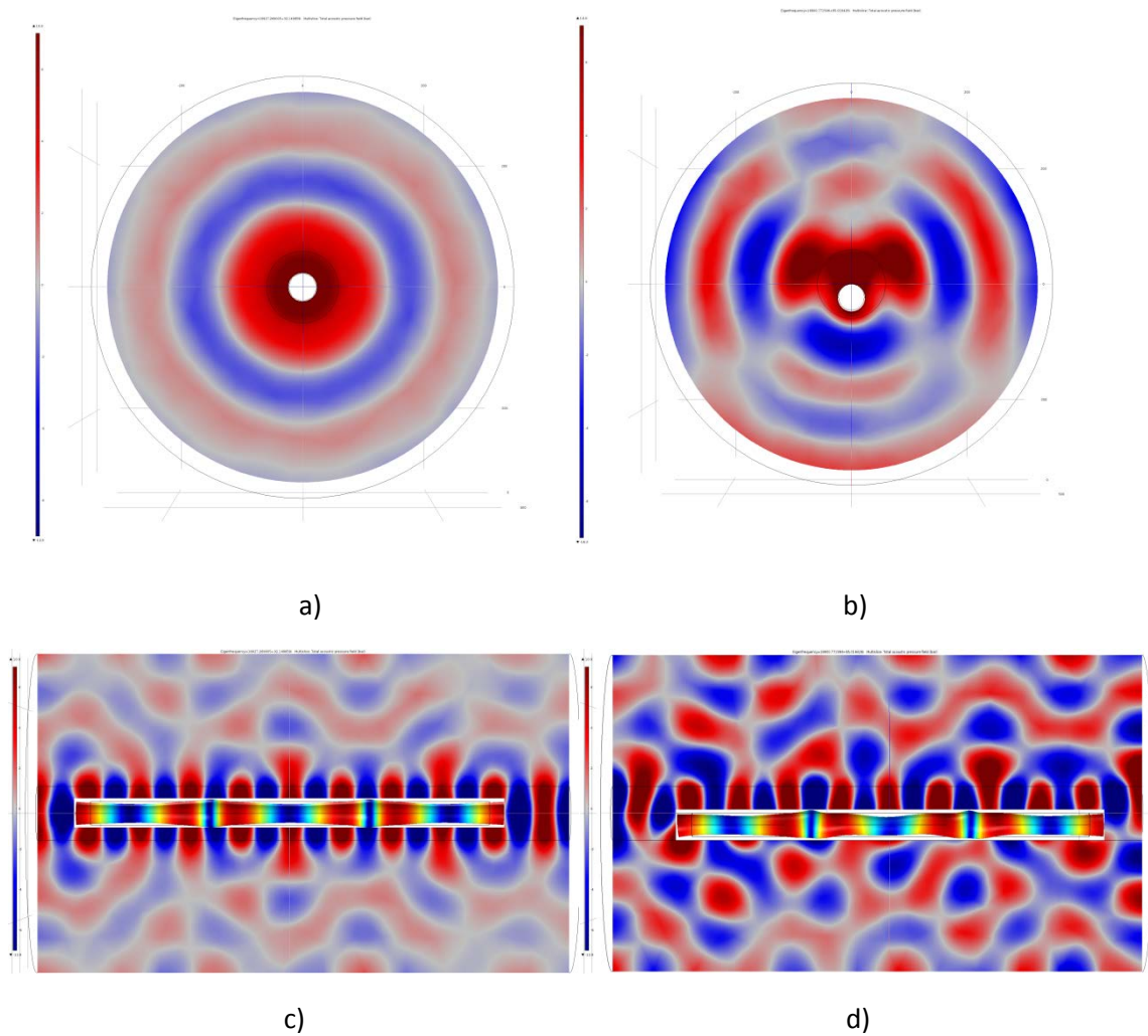
Fig. 5 Calculated interference patterns around the well
