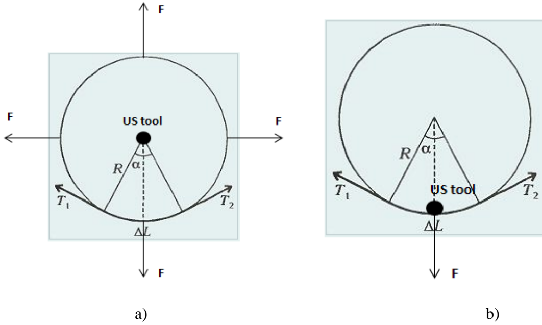
Fig. 6 Cross-sections of the model of the well in two cases: a) central position of the ultrasonic downhole tool; b)
