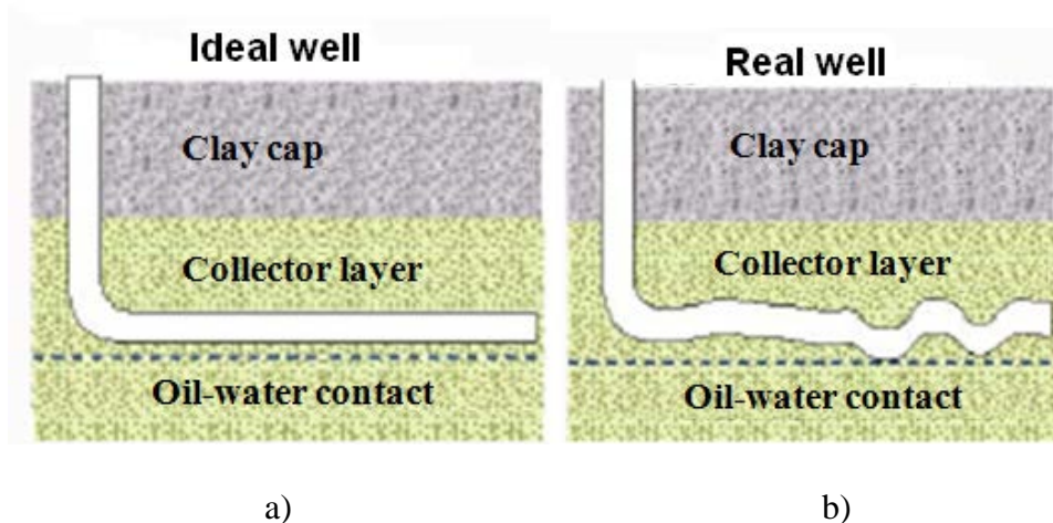
Fig. 2 Schema of ideal (a) and example of real (b) horizontal well
